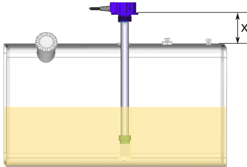
Figure 14: Calculating Extended Length
