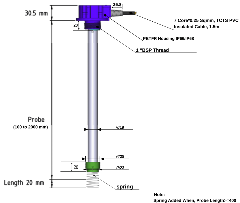
Figure 4: GA Drawing of Capvel-FUEL
