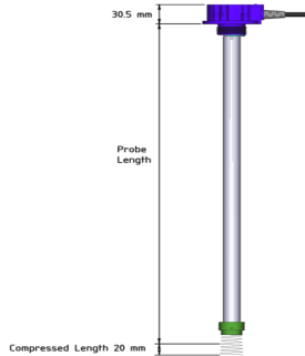
Figure 13: Calculating Probe Length
