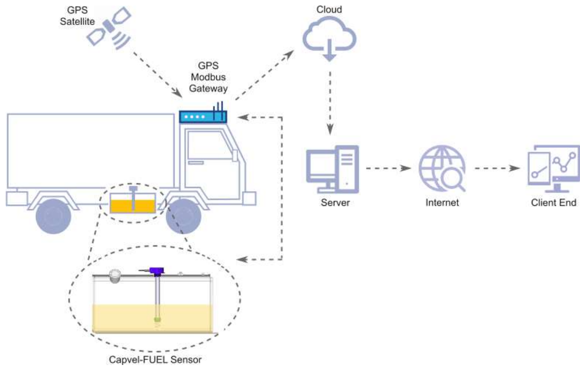
(a) System Architecture for Vehicle Tracking Systems
