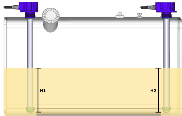
Figure 12: Tank Parallel to the Ground
