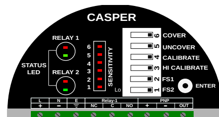
Figure 36: LED Indication on Top Cover
