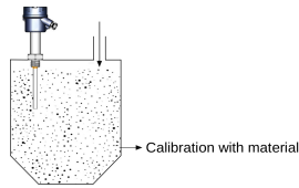
Figure 56: Calibration for Conductive Material
