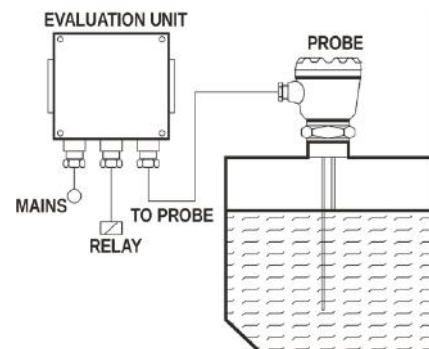
Figure 3: System Diagram
