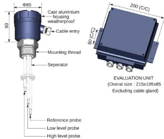
Figure 2: Part Diagram
